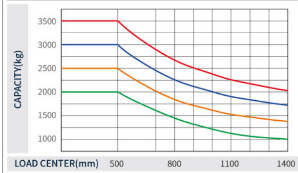
Load curve
